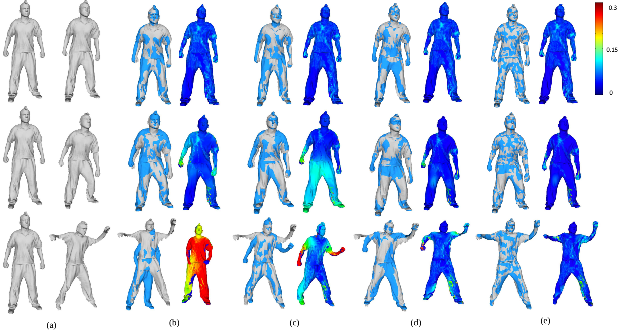
Figure 12. Registration results on Bouncing whole-to-part dataset with deformation degree increases from top to bottom: (a) Template and target, (b) ICP + \ell_0 -norm method [17], (c) Diffusion pruning (DP) + \ell_0 -norm method [17], (d) The SNR method [40], and (e) Our method.
